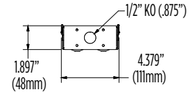
END VIEW
