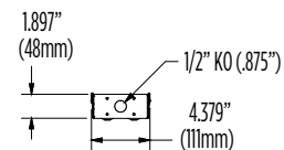
END VIEW
