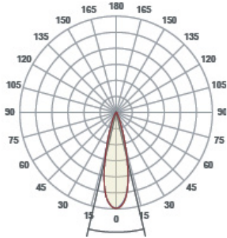
Beam Angle: 27°
