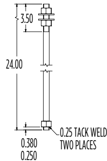
3/4x24 Steel Anchor Bolt 3/4x24 Galvanized Anchor Bolt
