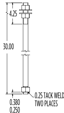
1x30 Steel Anchor Bolt 1x30 Galvanized Anchor Bolt
