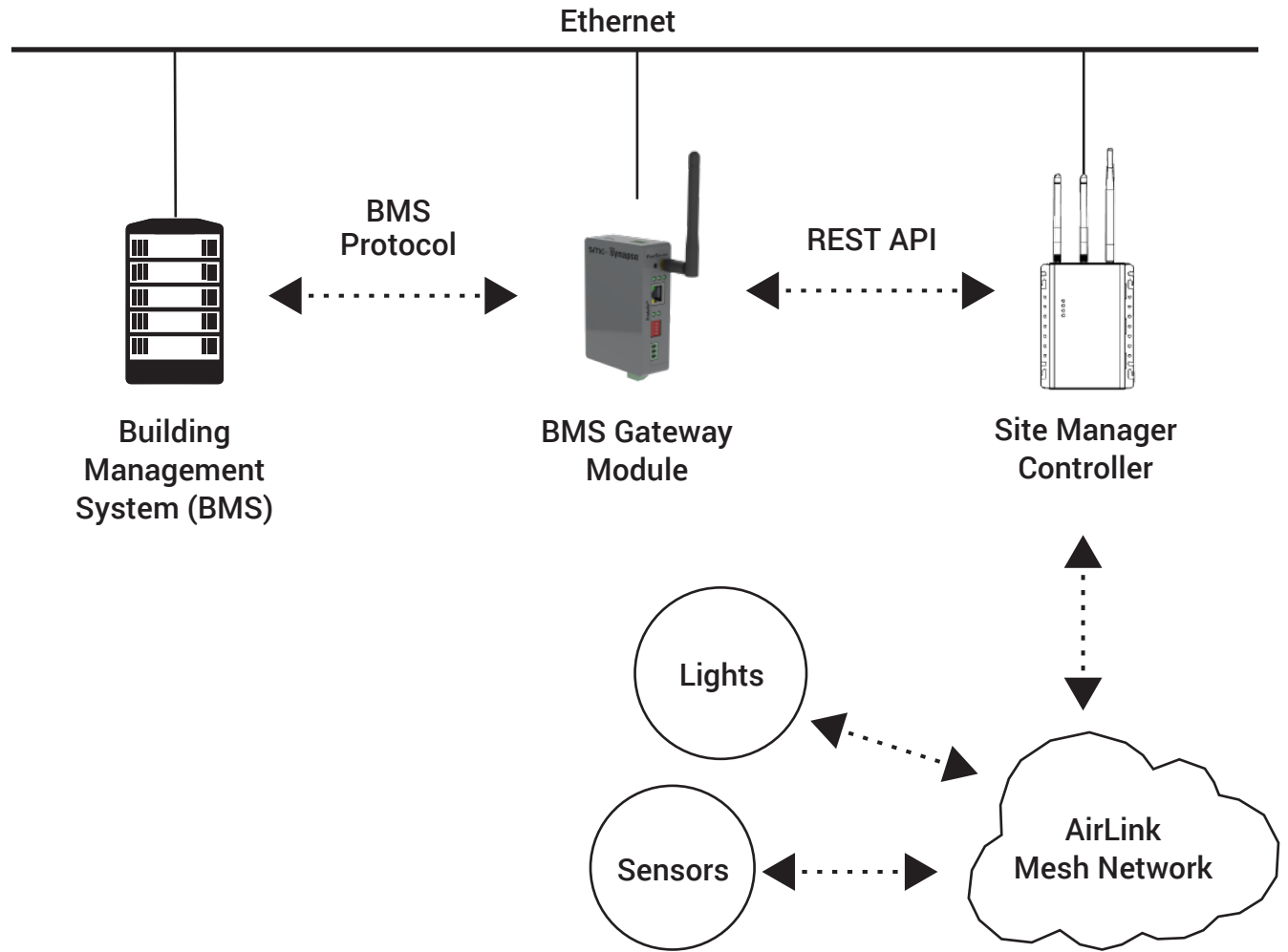
Example Setup of a BMS/AirLink Integration
