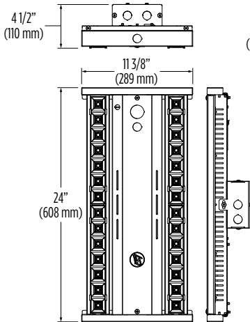
Zone Court Linear Low Glare, 2ft, 2 Row with Pendant Mount J-Box Kit (ZCL LG 2 12L-18L PMK)
