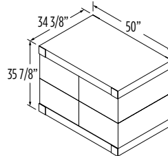
ZCL LG 24L/30L/36L 1 Pallet Position
