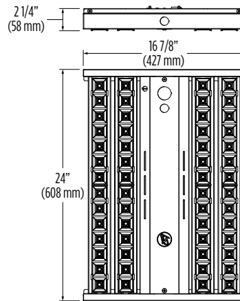
ZCL LG 24L/30L/36L 1 Pallet Position
