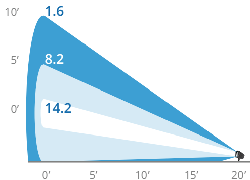
FOOTCANDLES ON THE TARGET
