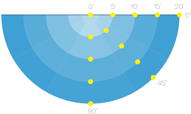
FOOTCANDLES ON THE GROUND
