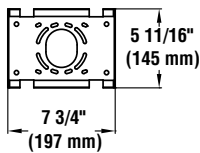
Universal Mounting Plate
