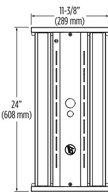
ZCL 24L/30L/36L 1 Pallet Position
