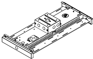
Zone Court Linear, 2ft, 2 Row with Pendant Mount J-Box Kit (ZCL 2 12L-18L PMK)
