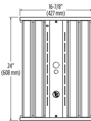
ZCL 48L/60L/72L 1 Pallet Position
