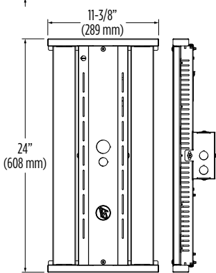
ZCL 12L/15L/18L 1 Pallet Position
