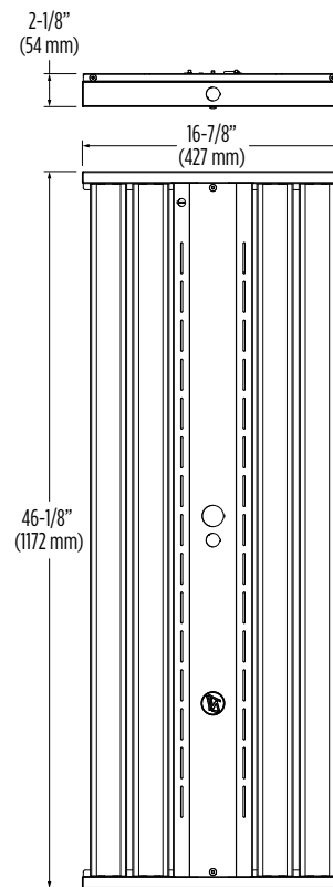
Peak Series High Bay, 4ft, 4 Row (PSHB 4 48L-72L)
