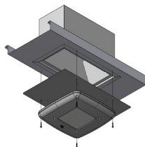
RECU Accessory Kit (731041) Includes cover panel, guide panel, tether clip and hardware
