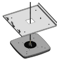
UNV Accessory Kit (731042) Includes mounting panel with auxiliary latch, 4 inner flange brackets and hardware to attach panel to fixture
