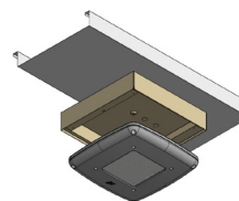
Surface Mount Box Kit (731043) Includes 2" deep housing with tether kit, tether bolt and mounting bolts.
