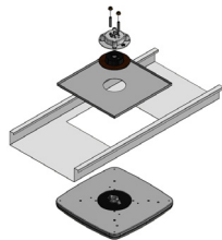
Encore 16" Accessory Kit (731039) Includes: top panel with sealant
