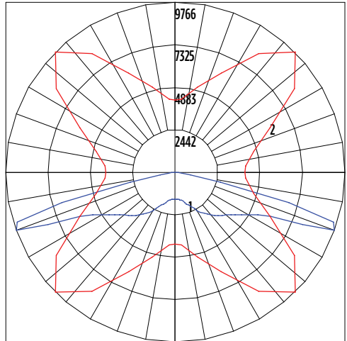
Polar Curve
