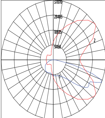
Polar Curve
