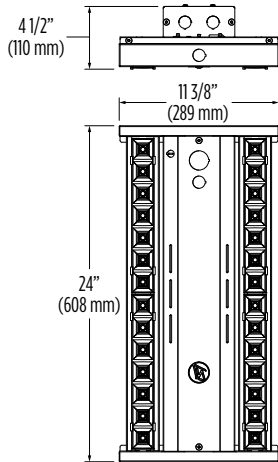
Zone Court Linear Low Glare, 2ft, 2 Row with Pendant Mount J-Box Kit (ZCL LG 2 12L-18L PMK)
