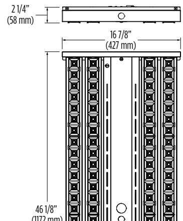
Zone Court Linear Low Glare, 4ft, 4 Row (ZCL LG 4 48L-54L)
