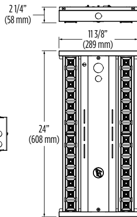
ZCL LG 12L/15L/18L 1 Pallet Position
