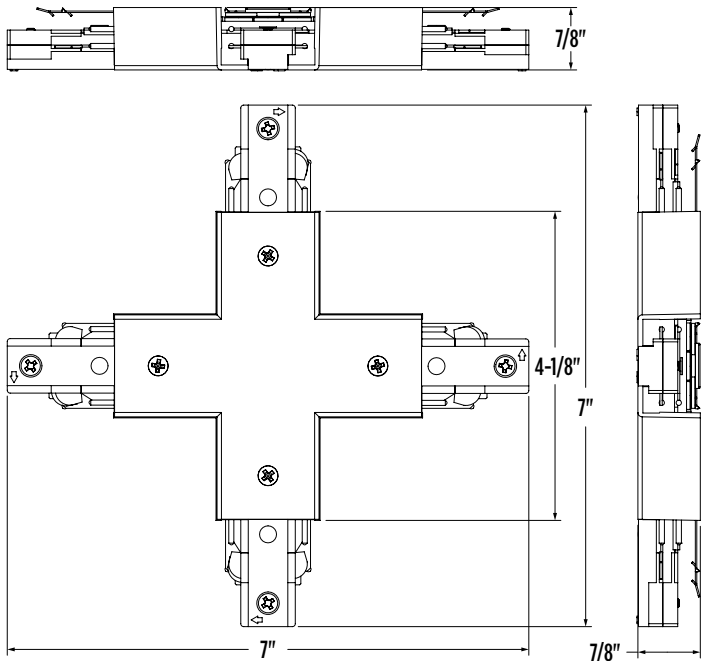
"X" Connector
