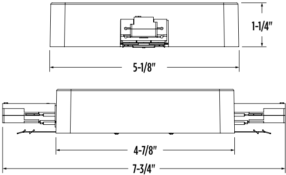
In-Line Feed Current Limiting Device (Housing Only)
