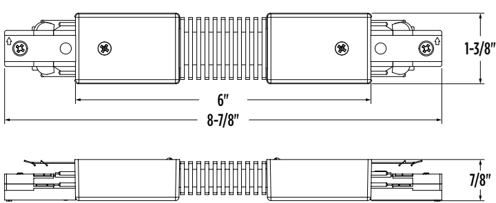
Flexible Connector
