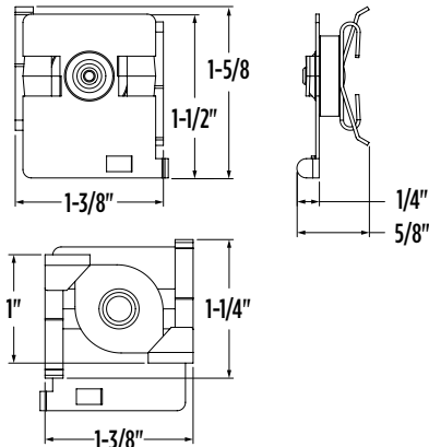
15/16 Inch T-Bar Surface Mounting Clip (Deep Tile)
