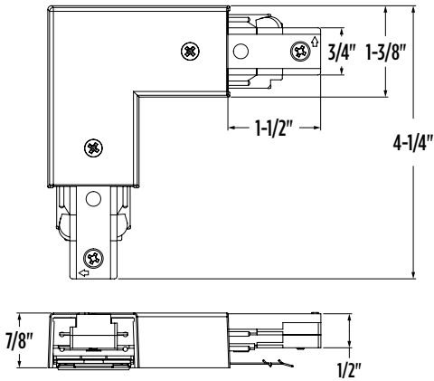
3-Way Connector
