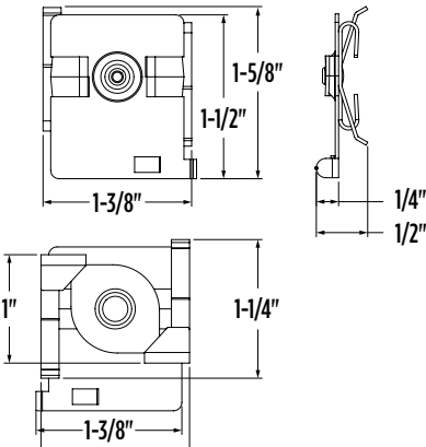
15/16 Inch T-Bar Surface Mounting Clip (Flush Tile)
