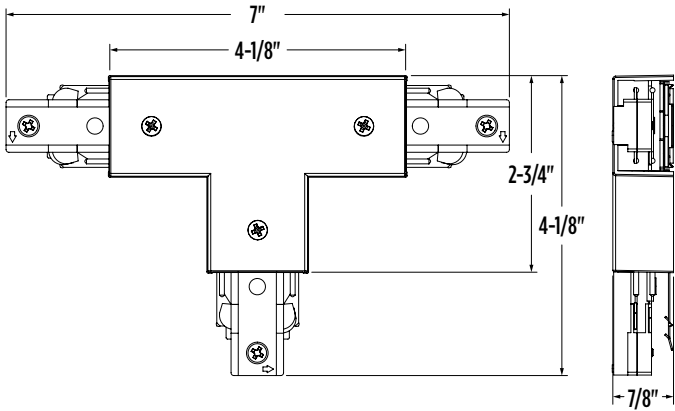
"T" Connector
