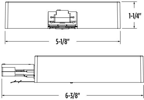
End Feed Current Limiting Device (Housing Only)
