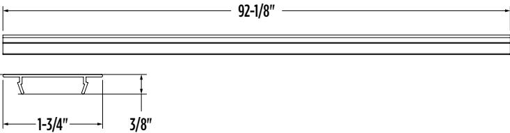
Decorative Track Insert
