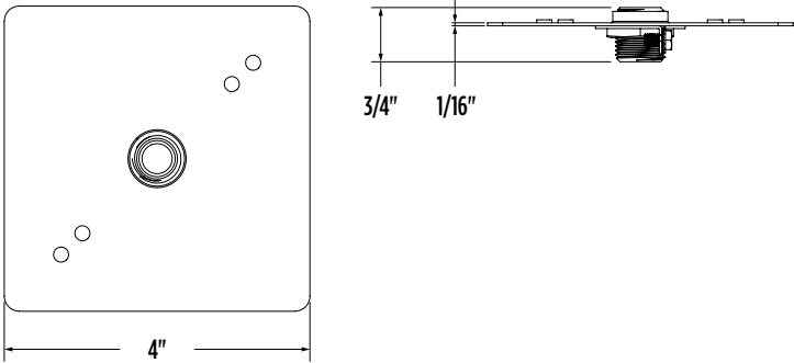
Outlet Box Cover Plate
