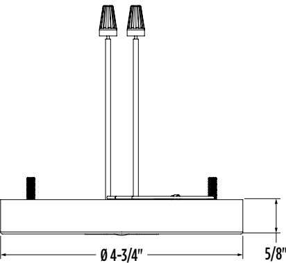
Line Voltage Mono-Point Adapter
