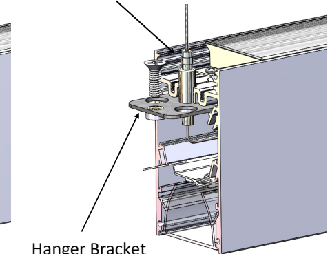
Hanger Bracket (Joining Fixture position)
