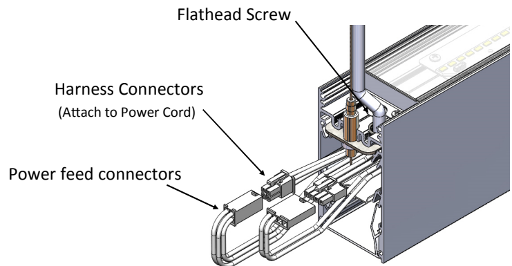
Hanger Bracket (End of Row position)
