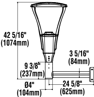
BK MPT BO Mount Optional D180 1.5G rated Arm Assembly Mounts to 4" or 5" Dia. D180 Bolt-on Pole Consult factory for alternate configurations
