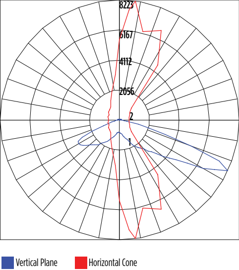
Polar Curve
