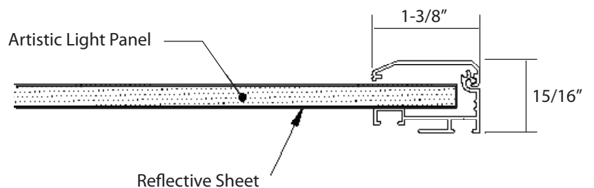
DETAIL SECTION
