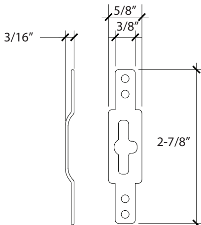
MOUNTING BRACKET
